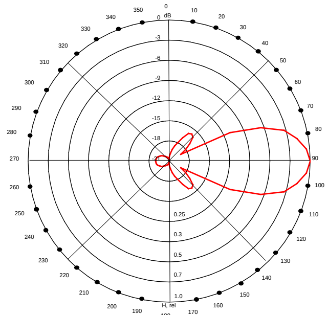
V pol - Vertical Radiation Pattern (E-Plane)
