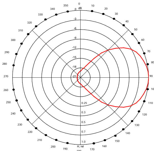
Vertical Radiation Pattern (H-Plane)
